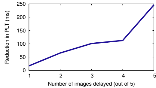
Figure 10: Relative benefits of pushing content for sites with a significant amount of computation, with 1-5 of 5 figures loading after the Javascript computation and the rest loading before.
